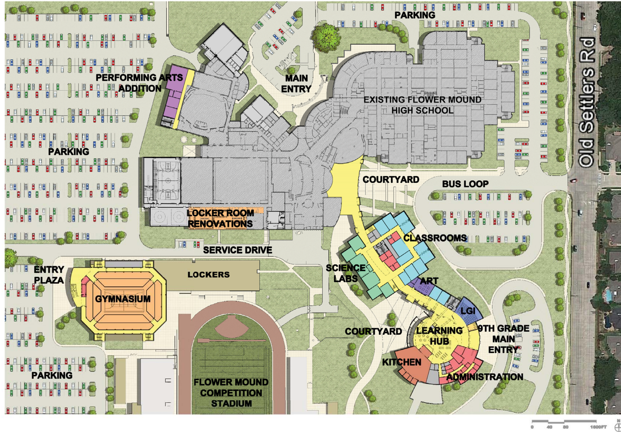
Composite Plan - First Floor
